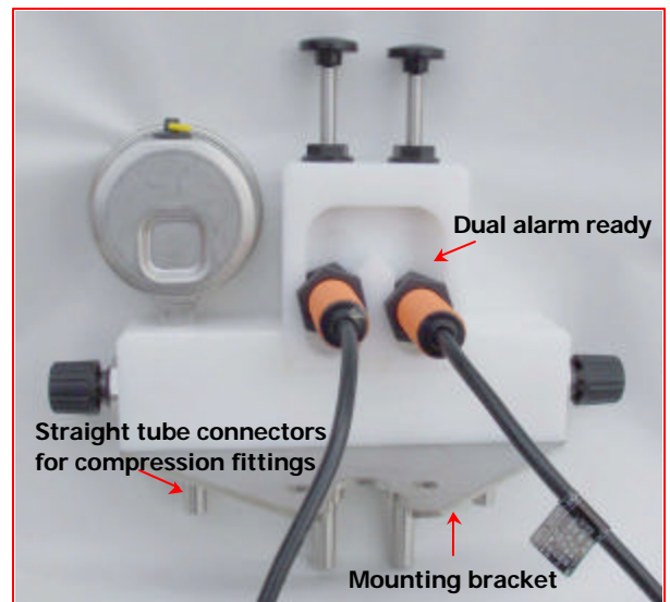
EDS Dual Seal Flowmeter
