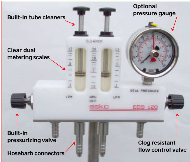
EDS Dual Seal Flowmeter
